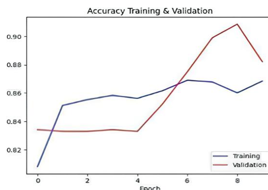
Fig. 5 Accuracy Graph of Training and Testing for the AlexNet Model
