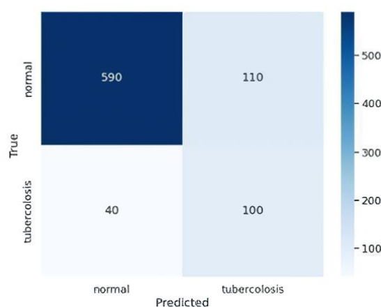
Fig. 12 Confusion Matrix ResNet
