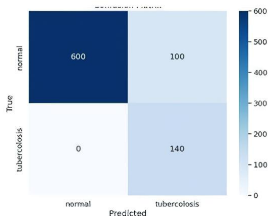
Fig. 11 Confusion Matrix AlexNet
